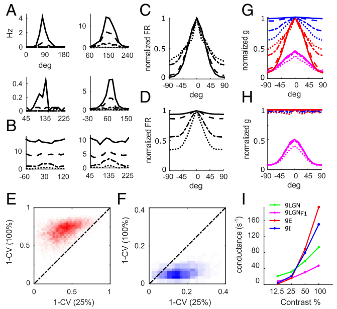
Fig. 2. Simulation results. Tuning curves of 12.5%, 25%, 50%, and 100% contrasts are in dotted, dot-dashed, dashed, and solid lines, respectively. ( A and B ) Examples of firing rate tuning curves of excitatory and inhibitory neurons, respectively. ( C and D ) Population averages of excitatory and inhibitory neurons' firing rate tuning curves, respectively. Every tuning curve is normalized by its maximum firing rate. ( E and F ) Heatmaps for the density distribution of 1 - CV with contrast at 25% vs. 100% for the firing rate tuning curves of excitatory and inhibitory populations, respectively. The dot-dashed line indicates contrast-invariant OS. ( G and H ) Population averaged, normalized tuning curves of conductances in excitatory and inhibitory neurons, respectively. The legend follows I . The total LGN conductance is not shown here, since it is flat and overlapped at y = 1 . Instead, we plot the F1 component of the LGN conductance (magenta) normalized to the F0 component. ( I ) Absolute levels of different conductances in the inhibitory population across contrasts corresponding to H , with averaged total LGN conductance in green.
